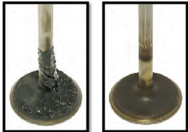
Photos of dirty (left) and clean (right) port intake valves
